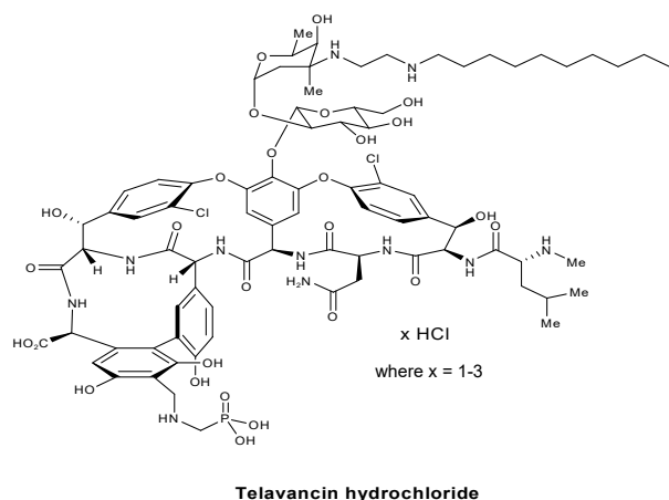
Figure 1: Telavancin Hydrochloride
