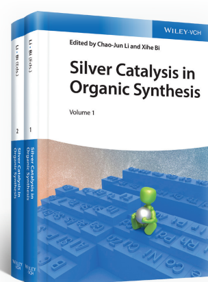
Silver Catalysis in Organic Synthesis
