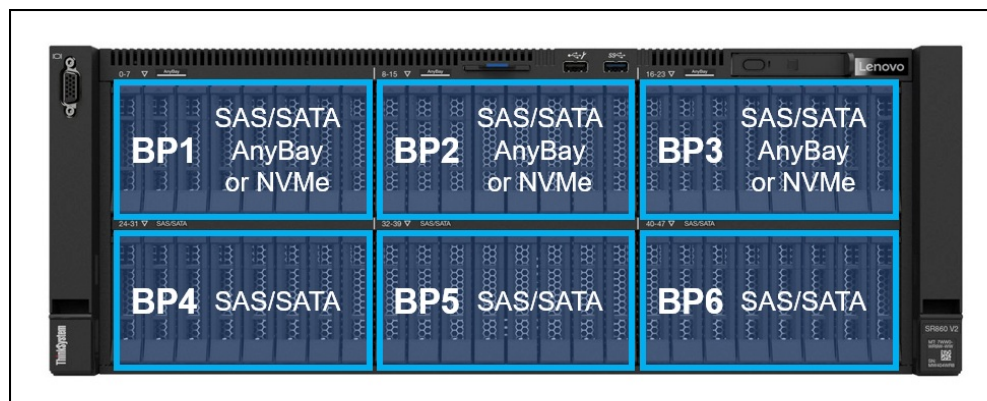
Figure 10. Backplanes
