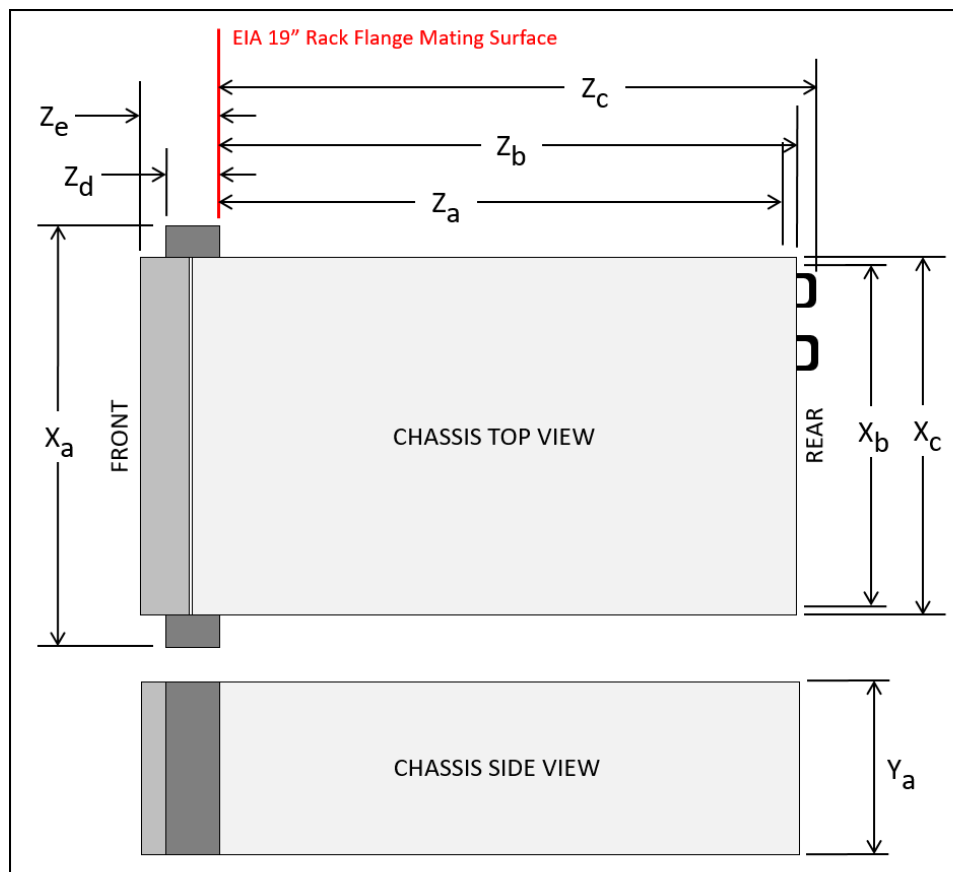
Figure 16. Server dimensions
