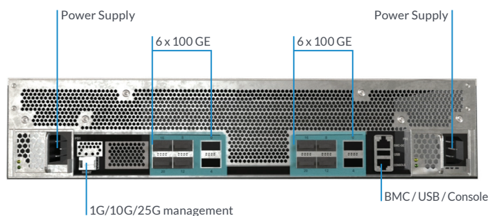
FS1600 Back Panel
